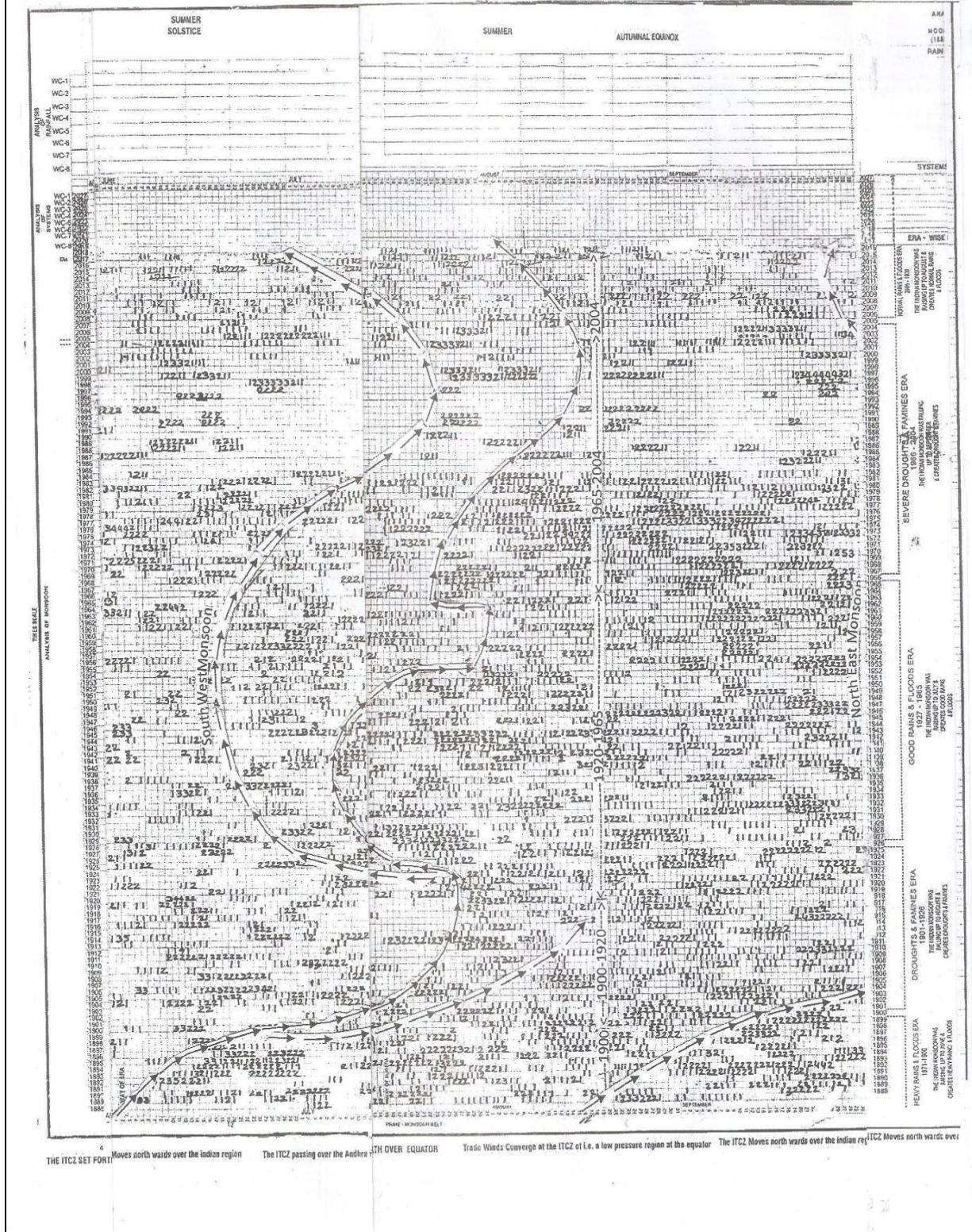
Indian monsoon time scales (when four parts are pasted)
