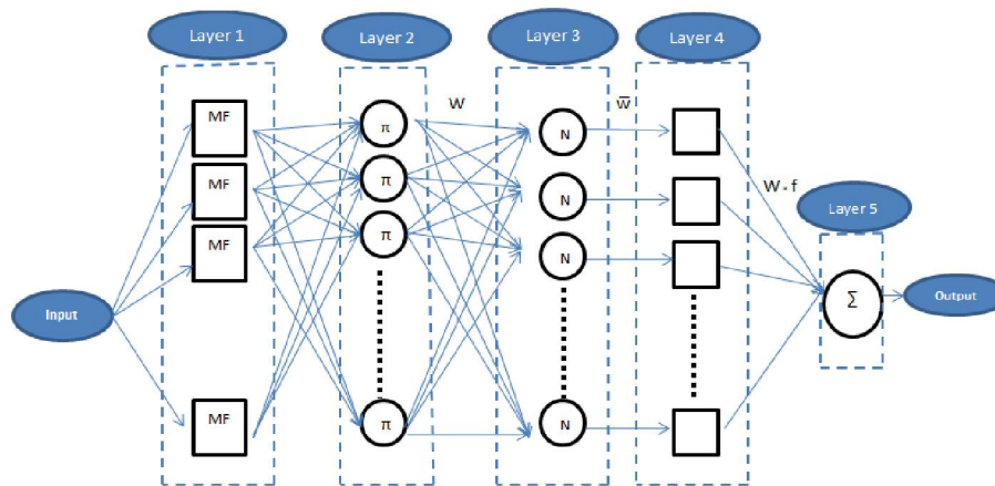
Fig. 3. Tagaki-Sugeno fuzzy model structure
