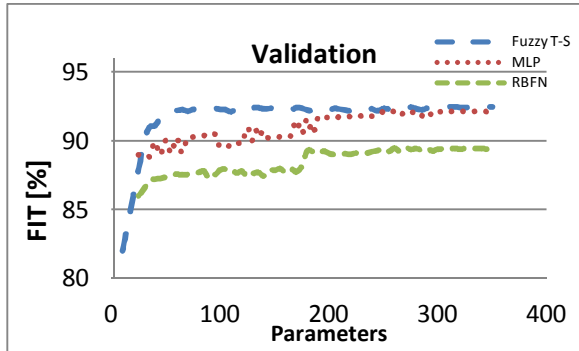
Fig. 7.b. Results of validation, T-S fuzzy model presented better validation performance
