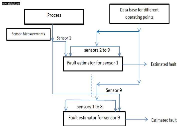
Fig.2. The proposed multiple fault tolerant measurement scheme
