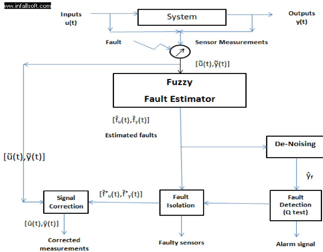
Fig. 2. The proposed multiple fault tolerant measurement scheme
