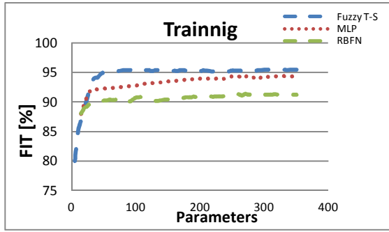
Fig. 7.a. Results of fitting performance, T-S fuzzy model showed the best performance
