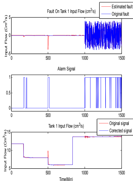
Fig. 8. Monte Carlo generated fault, Alarm and repaired signals for tank1 input water flow rate
