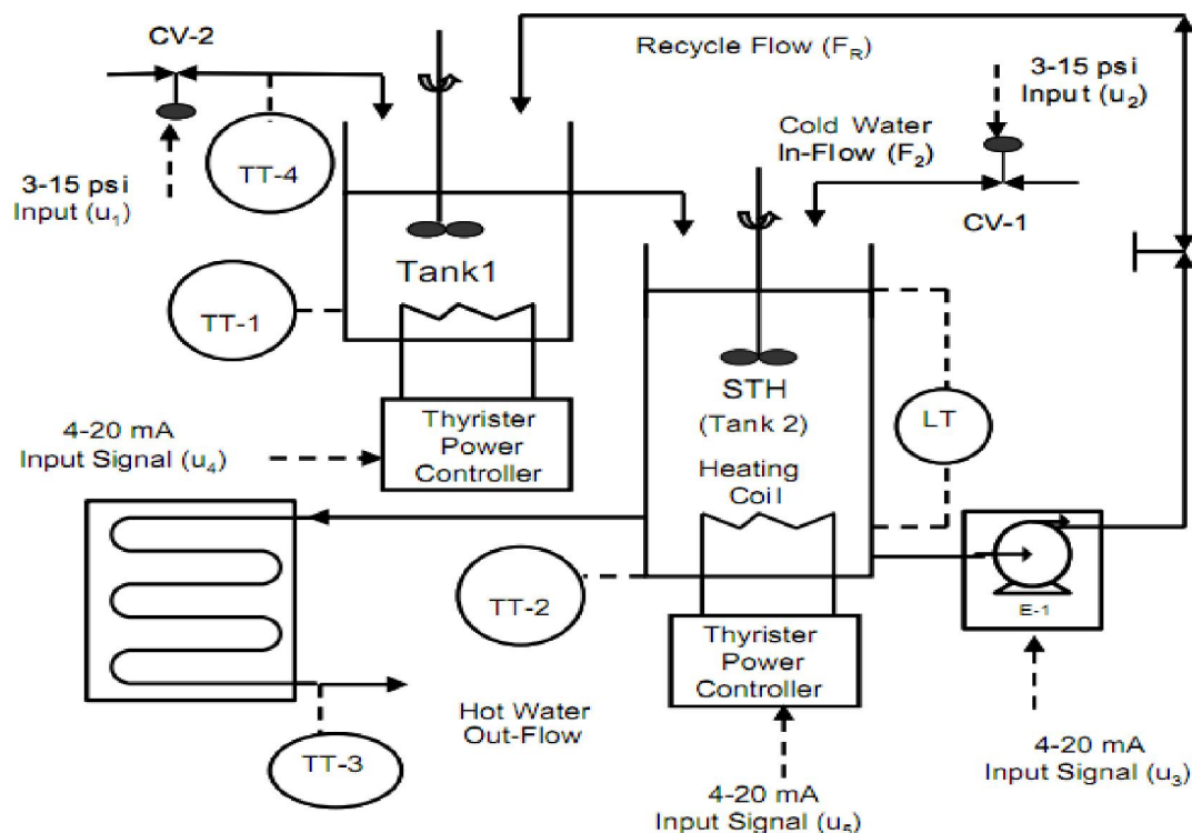
Fig.1 The continuous stirred tank heater (CSTH) [6]
