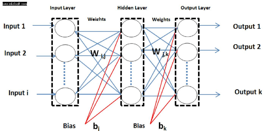
Fig. 5.b. MLP structure
