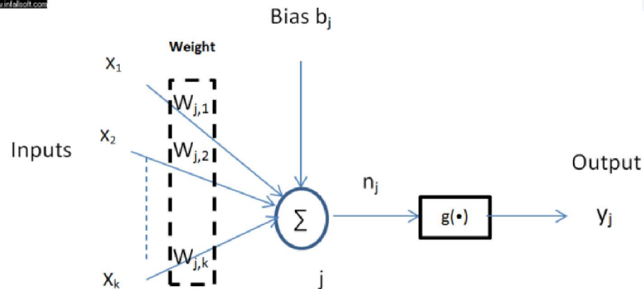
Fig. 5.a. Neuron structure
