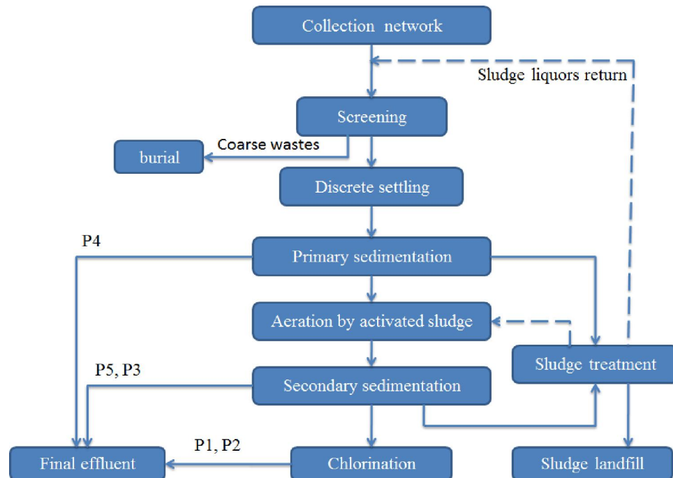
Figure 2. Schematic diagram of wastewater treatment processes used in studied units.
