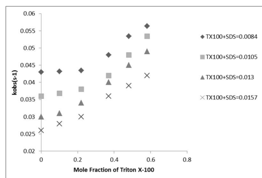
Figure 3: k_{obs} - X_{TX-100} profiles for the redox reaction of Malachite green at various fixed total concentrations of mixed surfactants. ( NO_2^- ) = 1.154 \times 10^{-3} \text{ mol dm}^{-3} and Temperature = 25.0 \pm 0.1^\circ \text{C}
