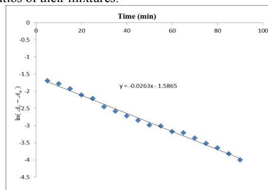
Figure 1C: Plot of \ln(A_t - A_\infty) versus Time (min) for the redox reaction of Malachite green and \text{NO}_2^- in mixed surfactant, [\text{MG}^+] = 5.77 \times 10^{-5} \text{ mol/dm}^3 , [\text{NO}_2^-] = 6.41 \times 10^{-3} \text{ mol/dm}^3 , \text{MG}_{D_o}^+ = 0.206 , \lambda_{\text{max}} = 620 \text{ nm} , [\text{SDS}] = 8.2 \times 10^{-3} \text{ mol/dm}^3 , [\text{TX-100}] = 2.28 \times 10^{-4} \text{ mol/dm}^3 , Temperature = 25.0 \pm 0.1^\circ \text{C} , A_\infty = 0.085 , Pseudo-first order rate, k_4 = 0.0606
