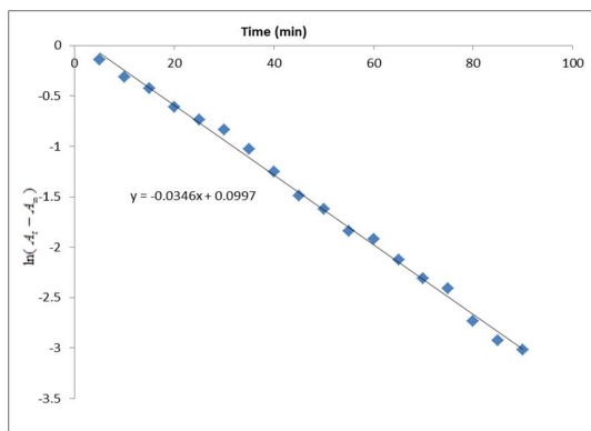
Figure 1B: Plot of \ln(A_t - A_\infty) versus Time (min) for the redox reaction of Malachite green and \text{NO}_2^- in SDS surfactant, [\text{MG}^+] = 5.77 \times 10^{-5} \text{ mol/dm}^3 , [\text{NO}_2^-] = 6.41 \times 10^{-3} \text{ mol/dm}^3 , \text{MG}_{D_o}^+ = 0.205 , \lambda_{\text{max}} = 620 \text{ nm} , [\text{SDS}] = 8.2 \times 10^{-3} \text{ mol/dm}^3 , Temperature = 25.0 \pm 0.1^\circ \text{C} , A_\infty = 0.063 , Pseudo-first order rate, k_2 = 0.0796
