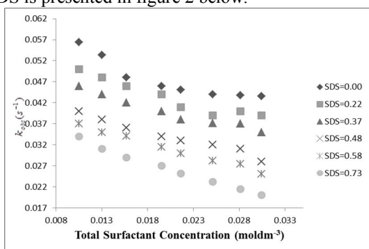
Figure 2: Variation of the observed rate constant ( k_{obs} ) as a function of the Total surfactant concentration for the redox reaction of Malachite green at various fixed mole fraction of SDS. ( NO_2^- ) = 1.154 \times 10^{-3} \text{ mol} / \text{dm}^3 and Temperature = 25.0 \pm 0.1^\circ \text{C}
