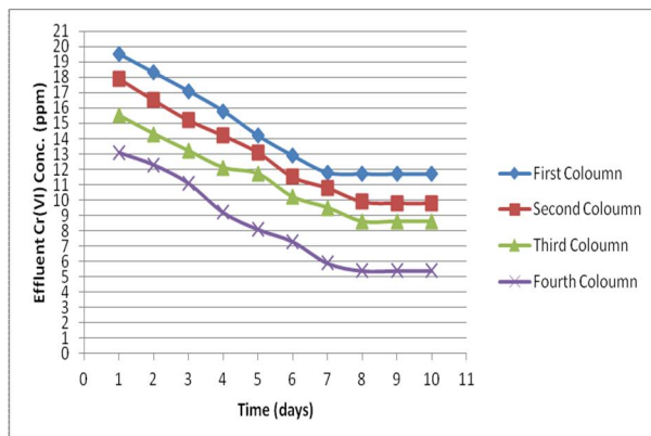
Figure (6) Time versus the effluent Cr (VI) concentration in Run III
