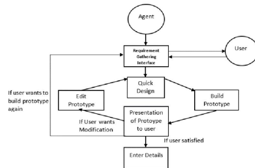
Fig 3: Automatic Prototyping through agents [28]
