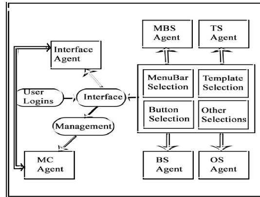
Fig 6: Working of Multi-Agent System
