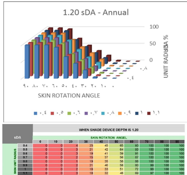
Fig. 4: (sDA 300/50% ) results of (1.20 m) depth.
