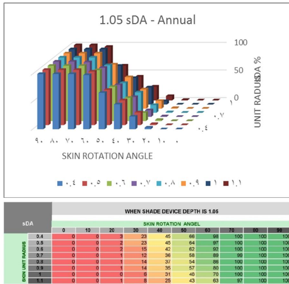
Fig. 6: (sDA 300/50%) results of (1.05 m) depth.
