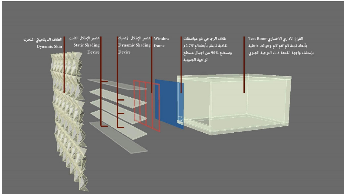
Fig. 1 Skin facade configuration.
