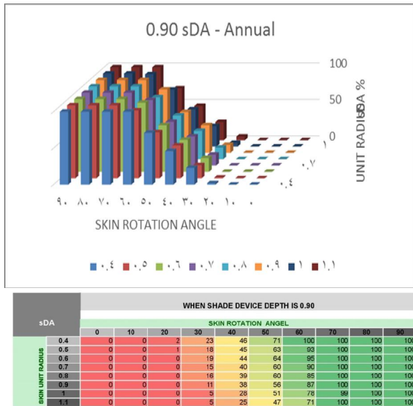
Fig. 7: (sDA 300/50%) results of (0.90 m) depth.
