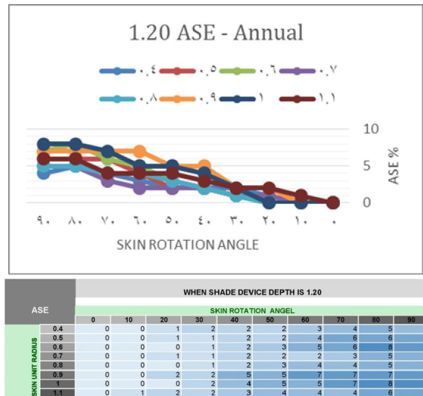
Fig. 5: (ASE 1000/250 ) results of (1.20 m) depth.
